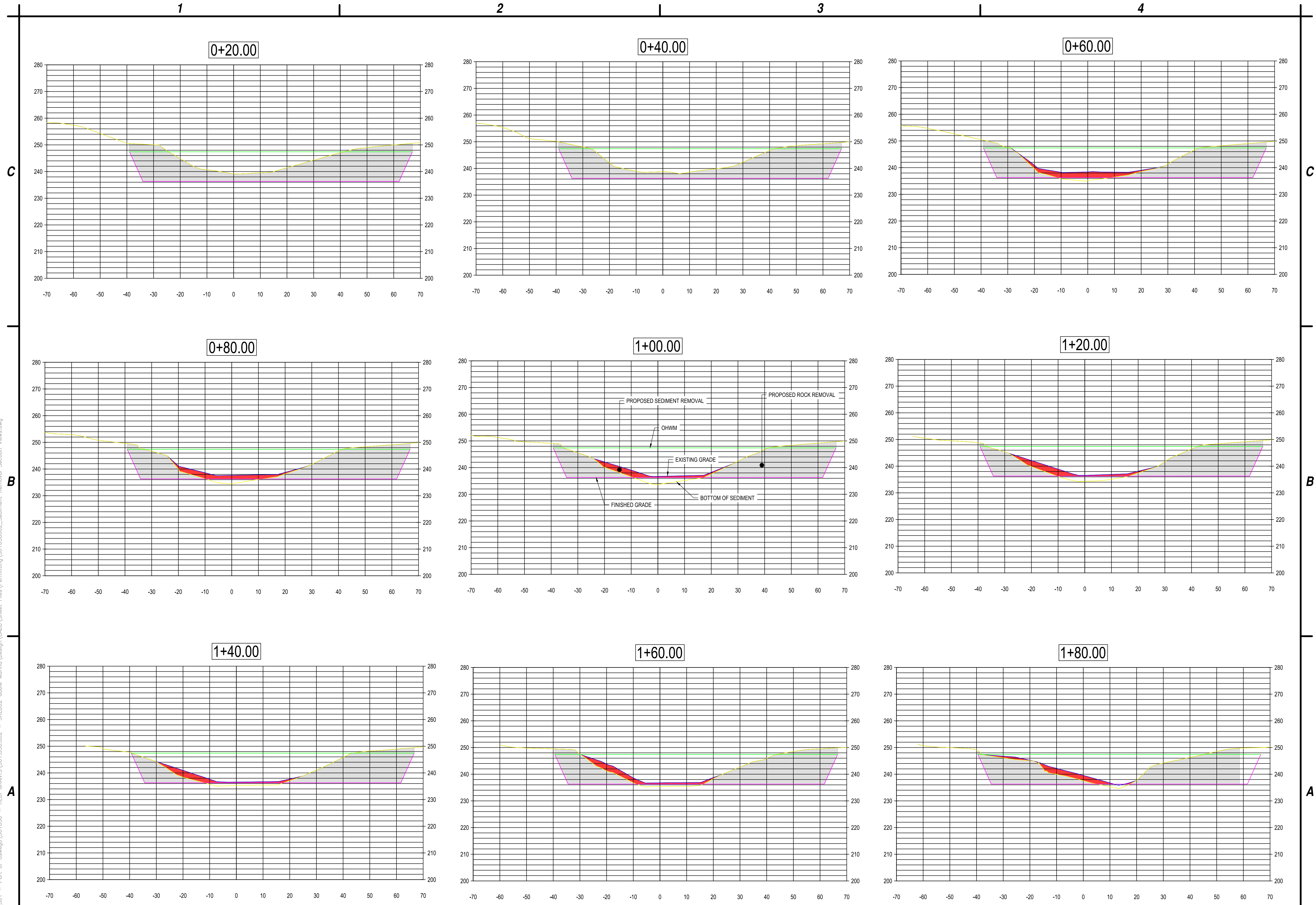
A1 SEDIMENT REMOVAL SECTION VIEWS SCALE: NOT TO SCALE
